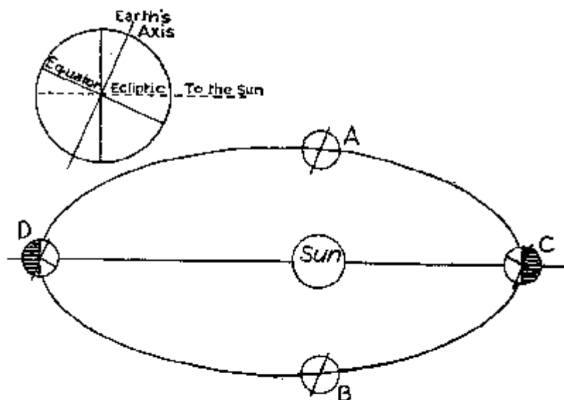
28. The earth's path around the sun. A and B show position of the earth on March 21st and September 22nd when day and night are of equal length. C and D show position of the earth on December 21st and June 21st, the shortest and longest days, of the year. The small diagram shows inclination of the earth's axis toward the sun on June 21st.
