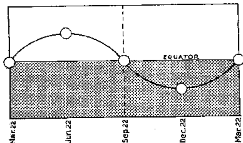
29. The diagram indicates the six months during which the sun rises north of the equator and the six months when it rises south of the equator, that is, when it is in the "Underworld."
