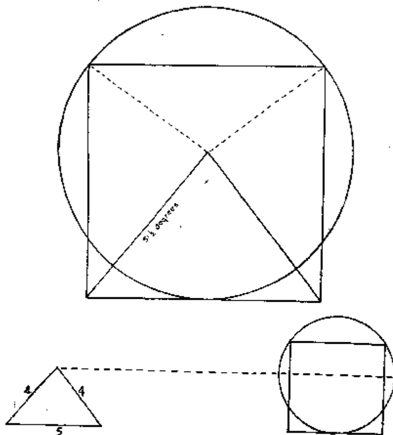
76. A 4 \times 5 \times 4 triangle as the basis for making a circle and square of approximately equal circumference. Lines from the center of the circle to the lower corners of the square have an angle of 5\frac{1}{2} degrees which is almost exactly the same as the sides of the Great Pyramid. Dotted lines in the large square at the top give the proportion of the flap on the apron of the Freemasons.
