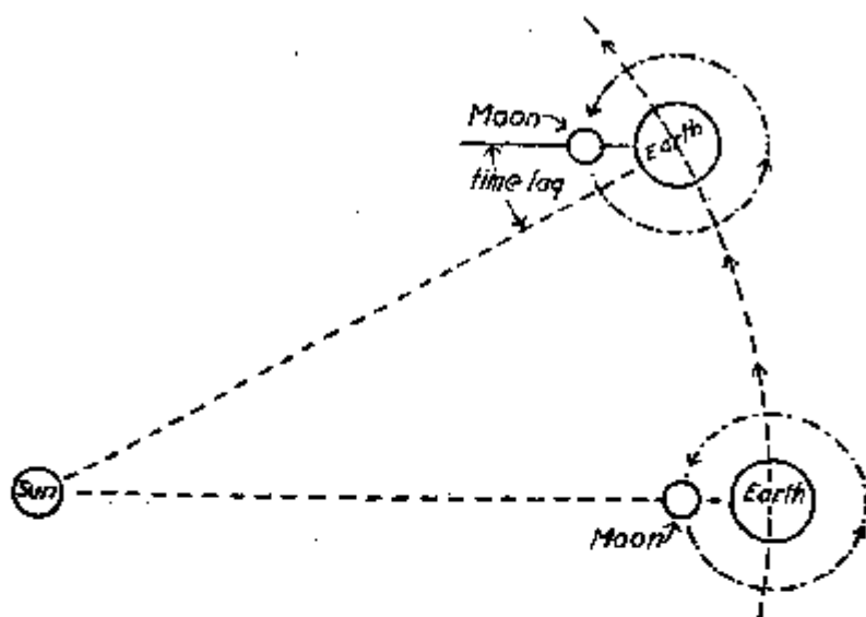
‡ Diagram showing why the moon has to make more than a complete revolution before returning to the same position relative to the sun and earth.
